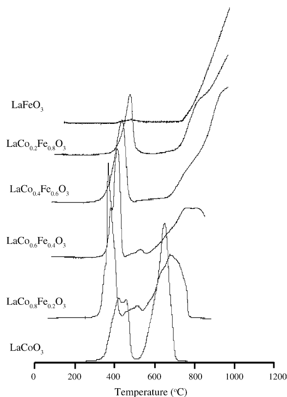
Fig. 2. TPR profile of \text{LaFe}_x\text{Co}_{1-x}\text{O}_3 mixed-oxide perovskite type series.
